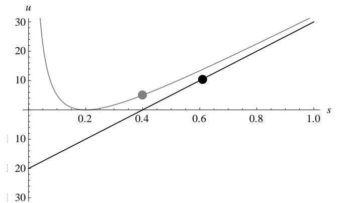
Fig. 2 Overall utility levels as functions of the overall revenue share for a=10c, b=1/2 , and c=1 .
