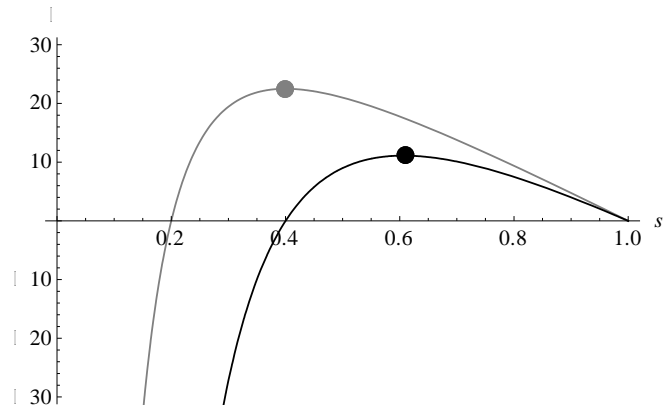
Fig. 1 Profit levels as functions of the overall revenue share for a=10c, b=1/2 , and c=1 .
